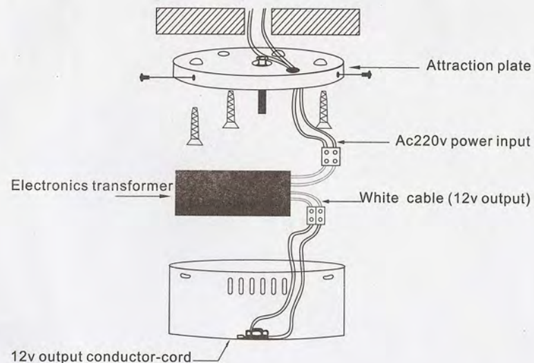
Transformer installing sketch diagram
